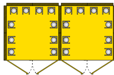
PAN 08 PANDESA 10+10 places W 3440 x D 1680 x H 2400 mm Weight: 909 Kg
